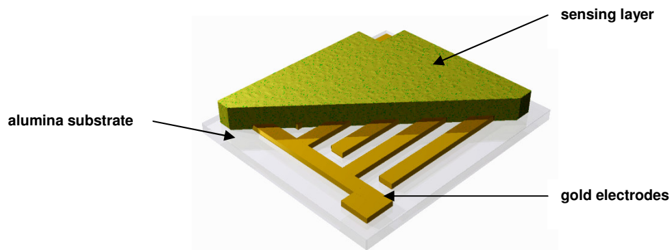
Diagram of typical sensor formulation
